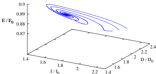
Figure 4: Projection of the unstable manifold of the N2_ML travelling wave solution.
